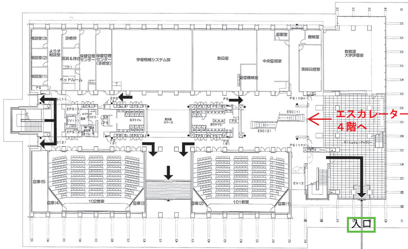
1階PLAN 1:400
